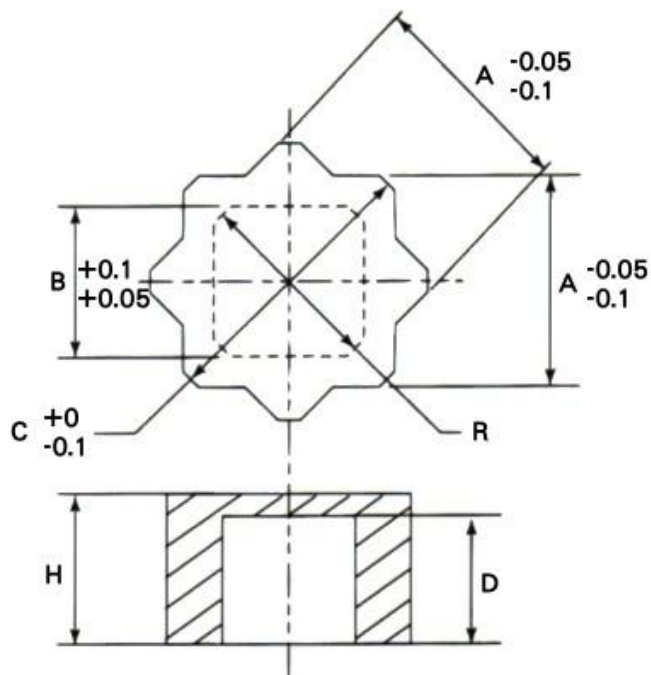
27M14 to 36M27 Design
